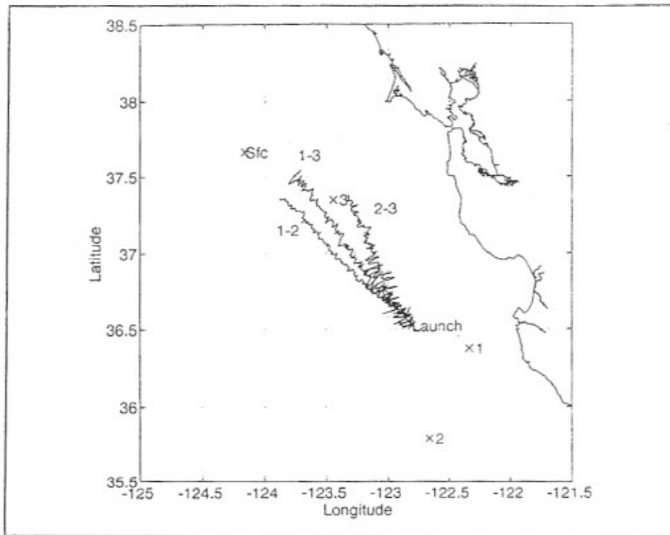
Figure 22. NPS #22 Two-Source (ARTRK) Solutions (source pairs indicated).
