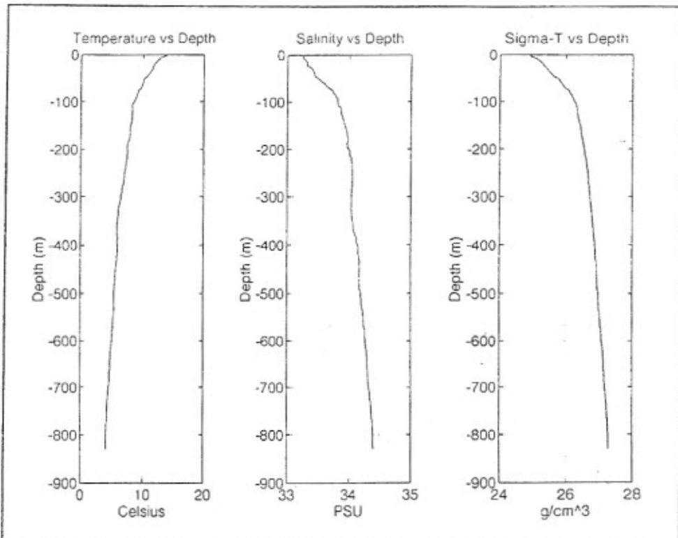
Figure 30. CTD Parameters (Source One). a) Temperature vs Depth, b) Salinity vs Depth, c) Sigma-T vs Depth.
