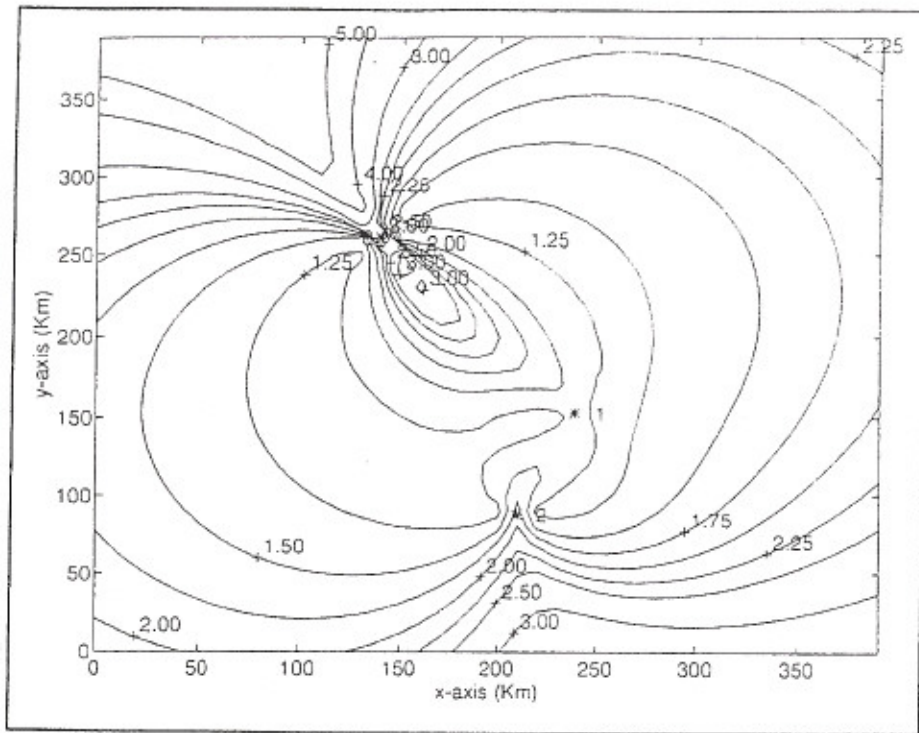
Figure 7. DOP Contour Plot for three sound sources.
