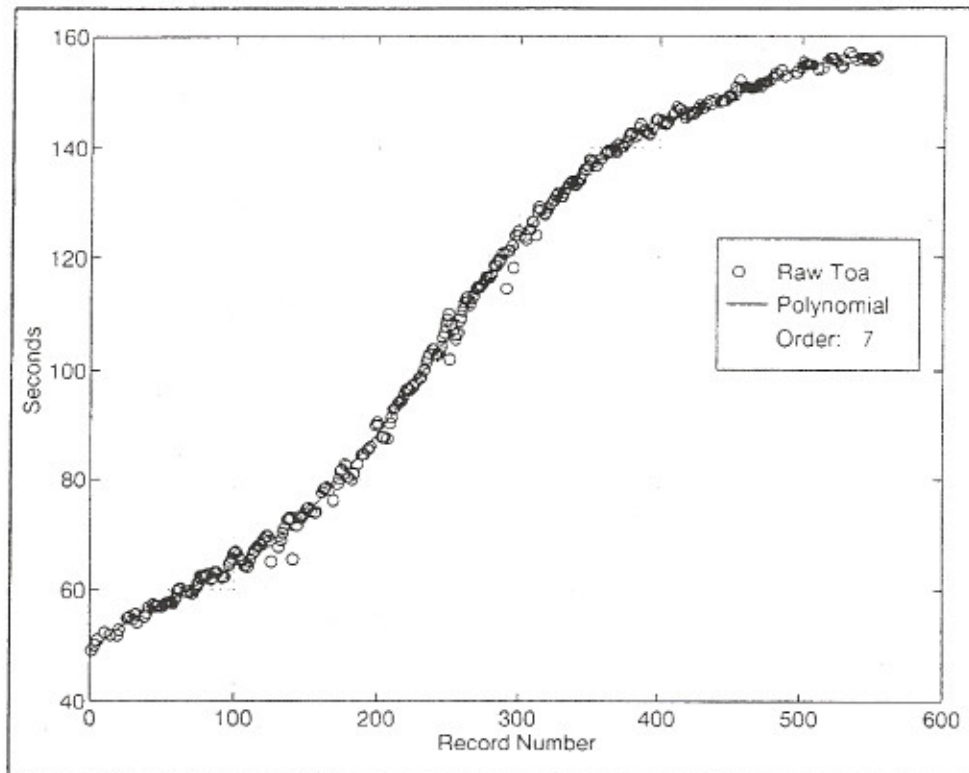
Figure 12. Seventh Order Polynomial fit to NPS #30 TOA Record from Source Two.
