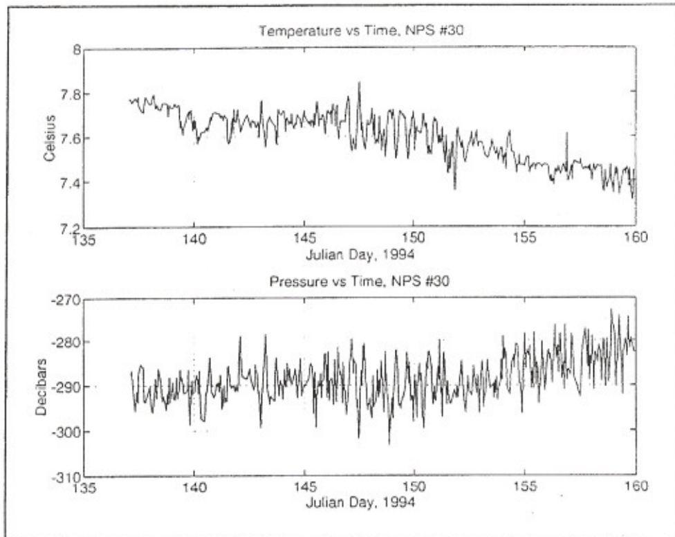
Figure 34. NPS #30 plot of temperature and pressure.
