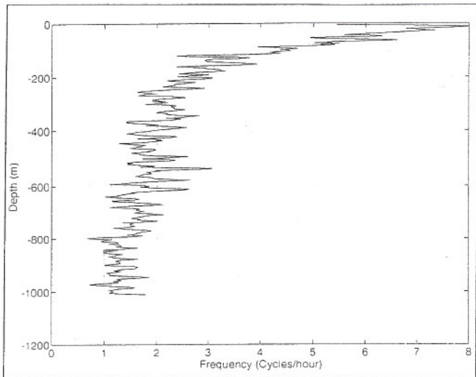
Figure 35. Average Buoyancy Frequency (Cycles per Hour).
