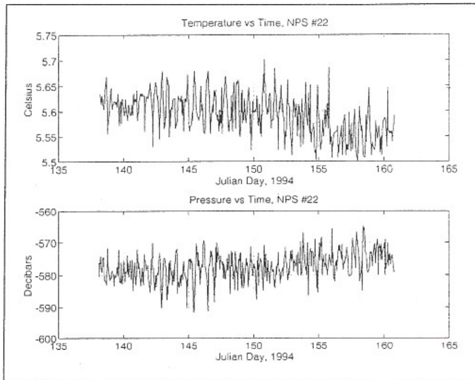
Figure 32. NPS #22 plot of temperature and pressure.
