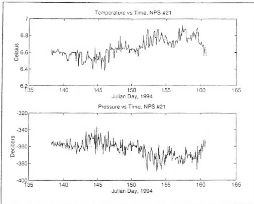
Figure 31. NPS #21 plot of temperature and pressure.
