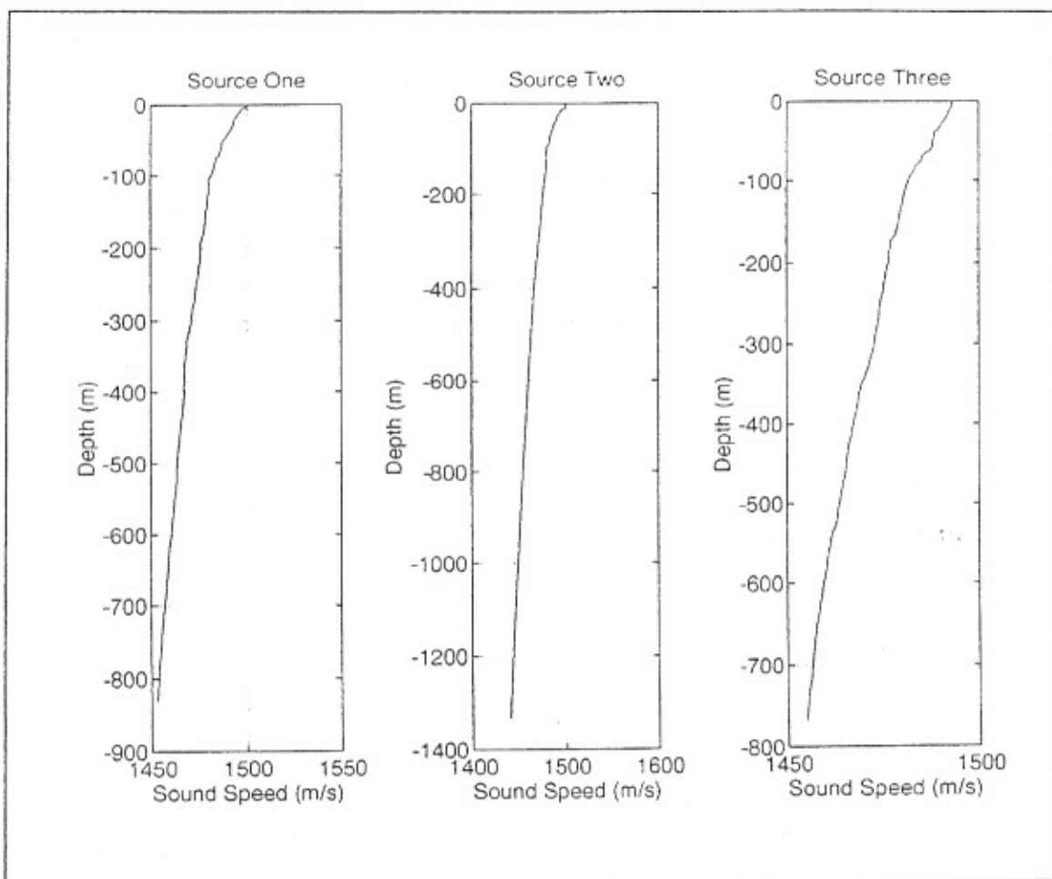
Figure 6. Sound speed profile versus depth at each source. a) Source One, b) Source Two, c) Source Three.
