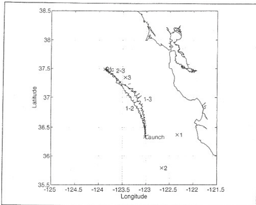
Figure 25. NPS #24 Two-Source (ARTRK) Solutions (source pairs indicated).
