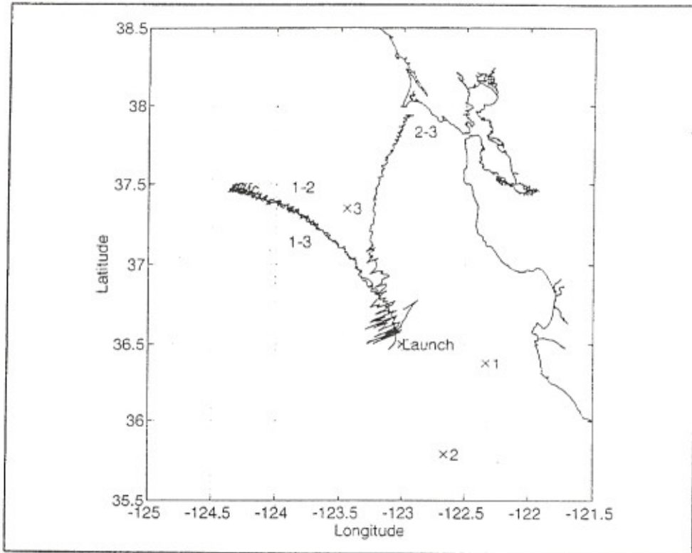
Figure 17. NPS #30 Two-Source (OMLS) Solutions (OMLS systematic error added) (source pairs indicated).
