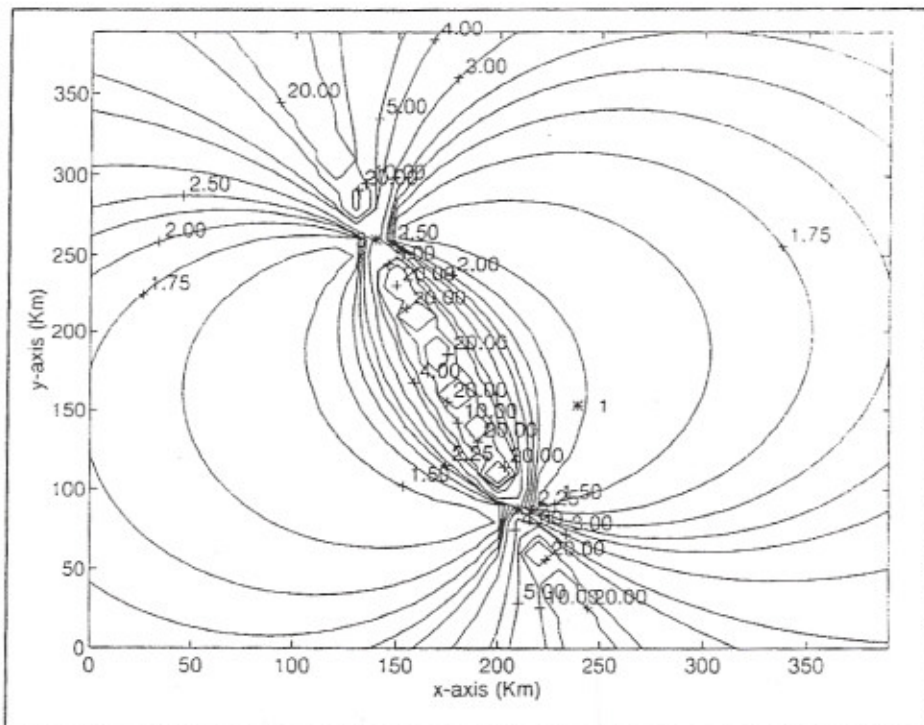
Figure 8. DOP Contour Plot for two sound sources. (Sources Two and Three).
