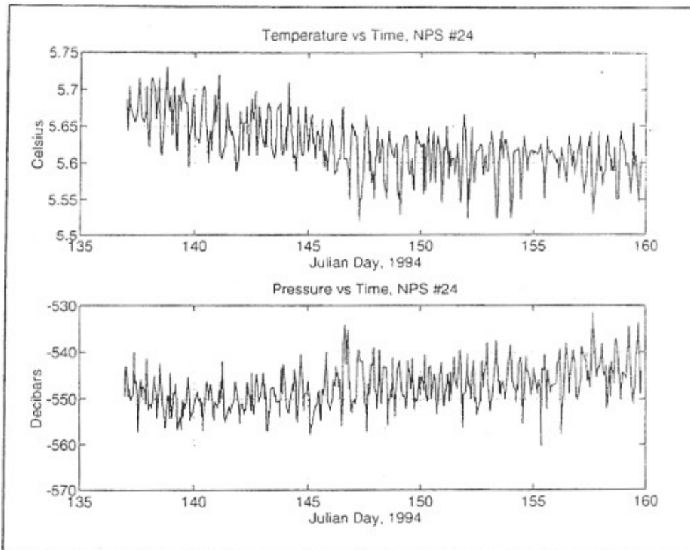
Figure 33. NPS #24 plot of temperature and pressure.
